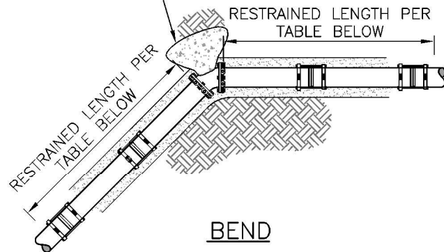
PVC & DI PIPE JOINT RESTRAINT SIZING TABLE REQUIRED RESTRAINT DISTANCE (FT.)
