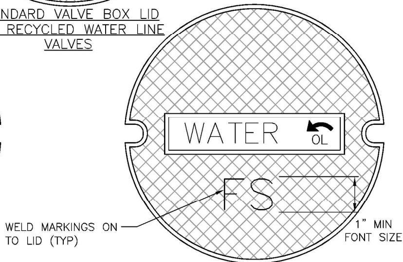
STANDARD VALVE BOX LID FOR ALL FIRE SERVICES
